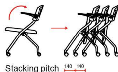
Stacking pitch 140 140
